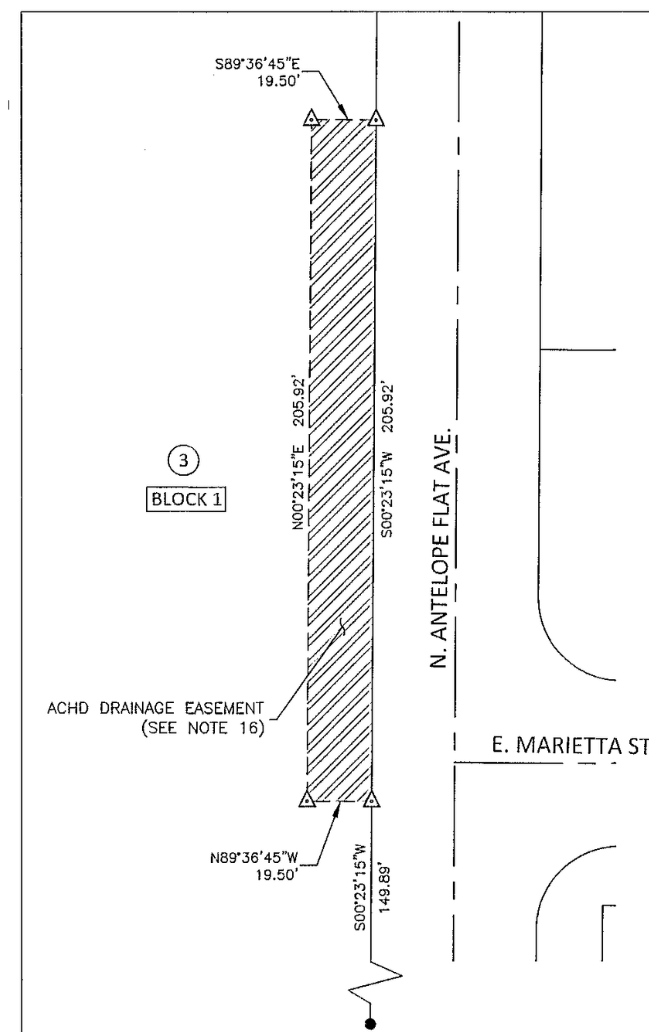
DETAIL C
