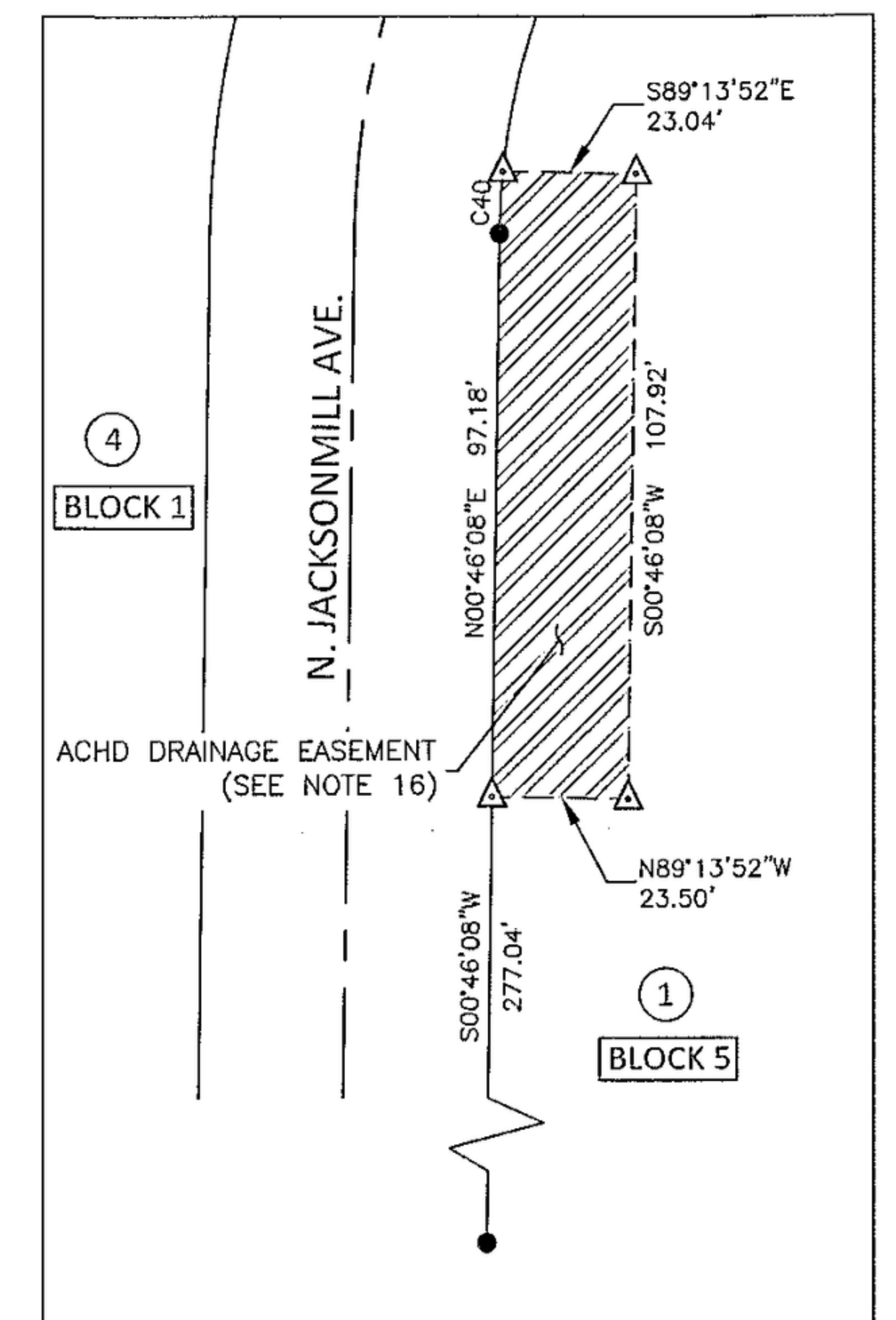
DETAIL B
