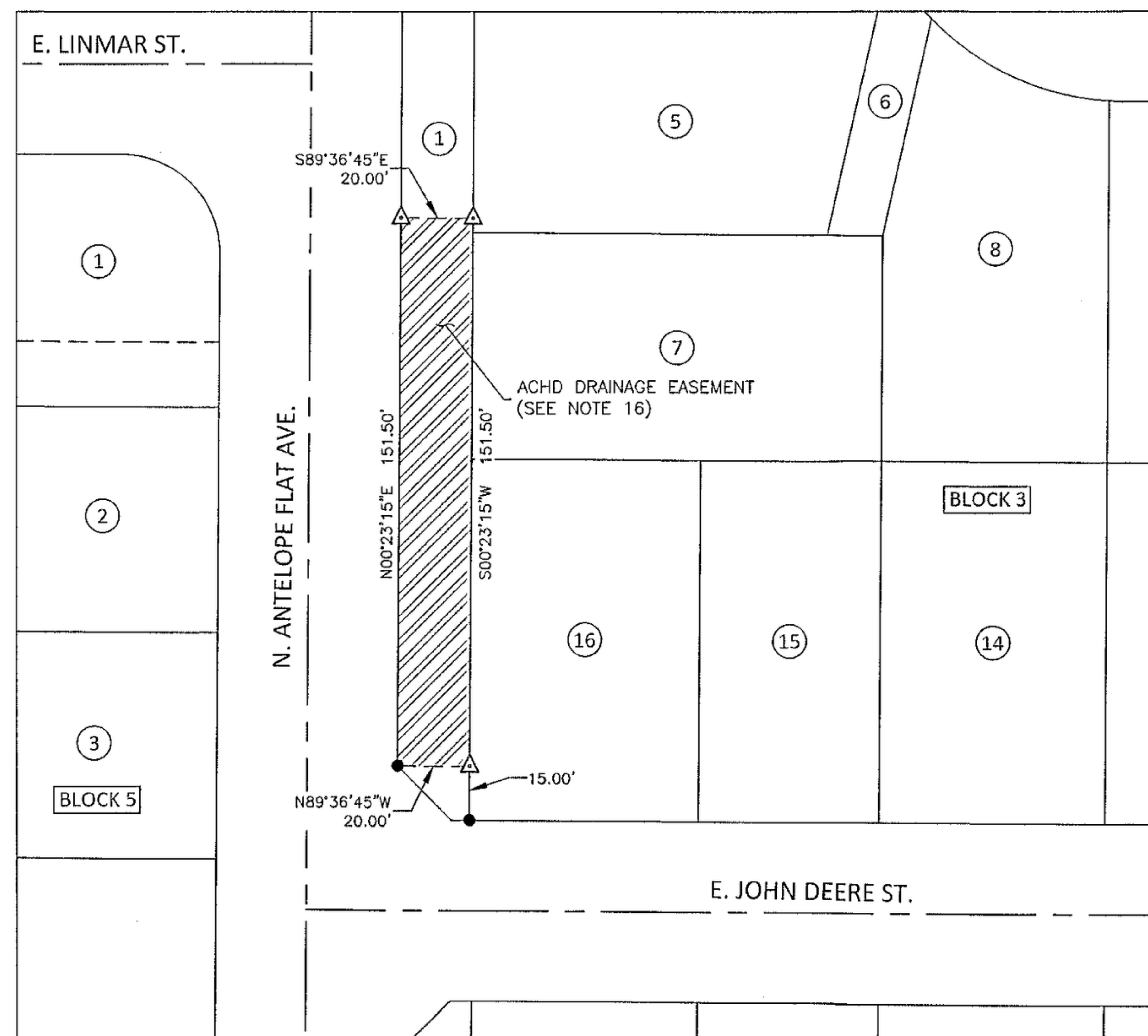
DETAIL D
