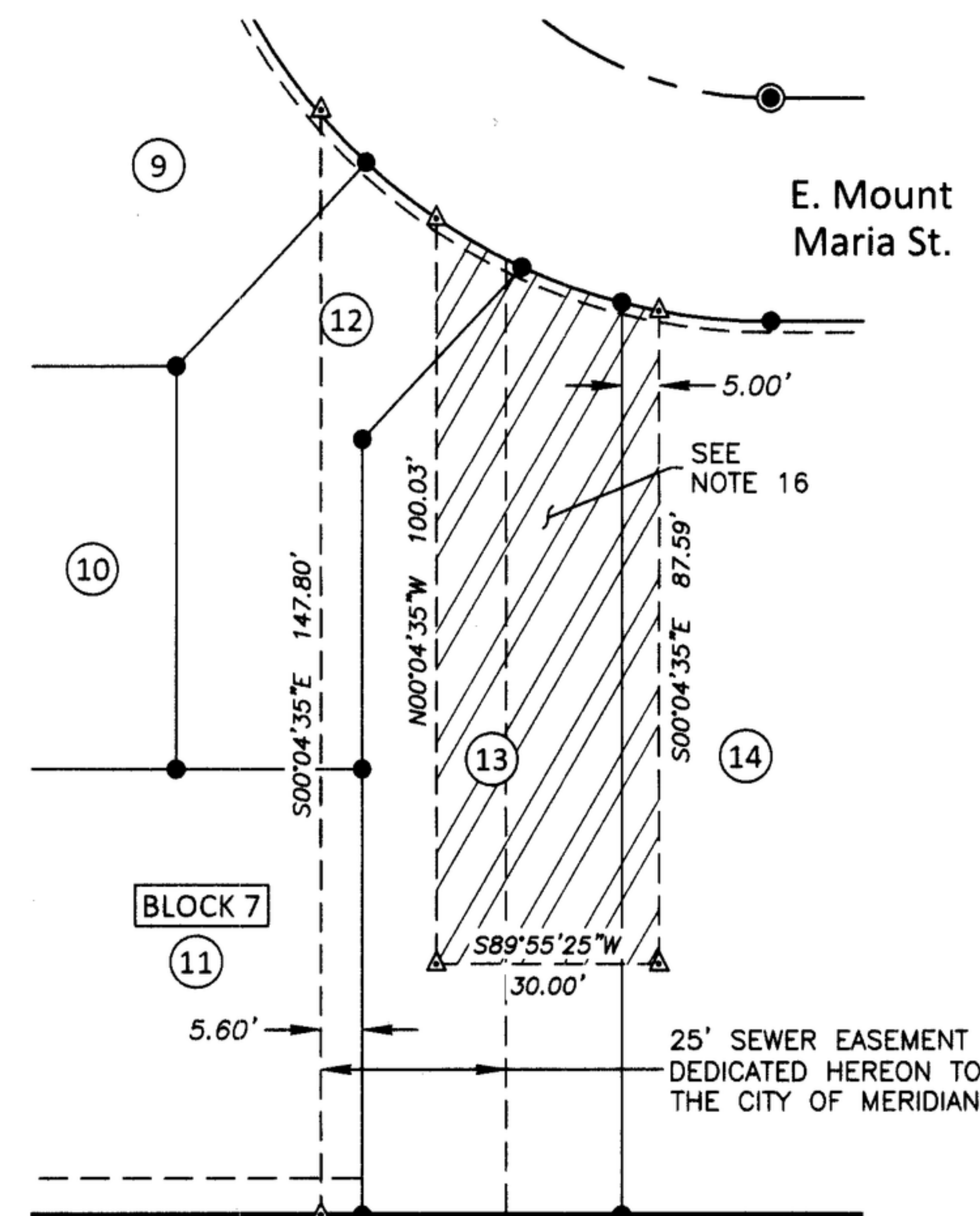
DETAIL "B" SCALE: 1"=30'
