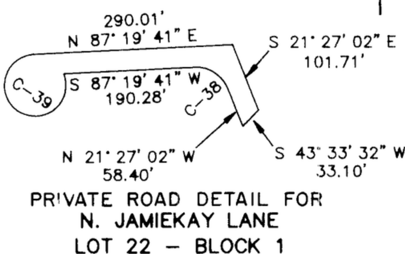
INGRESS-EGRESS EASEMENT DIAGRAM
